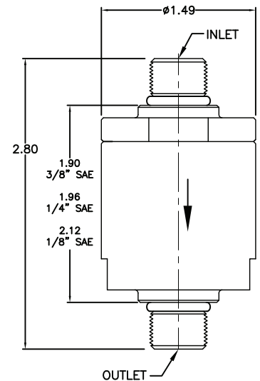
1/8, 1/4, & 3/8 MALE SAE
